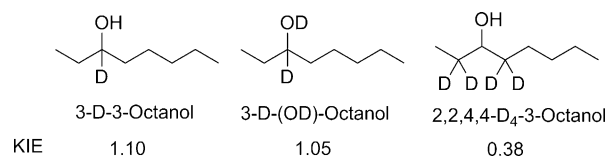
Scheme 1. Deuterated alcohol substrates for KIE experiments. Reaction conditions: NH 4 ReO 4 (0.2 mmol) and alcohol or deuterated alcohol (20 mmol) were mixed and refluxed at 180 °C for 180 min. Results are based on 1 H and/or 2 D NMR as the average of two runs.
