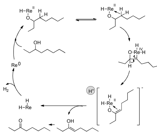
Scheme 2. Proposed acceptorless dehydrogenation (AD) of 3-octanol through γ-CH activation.
