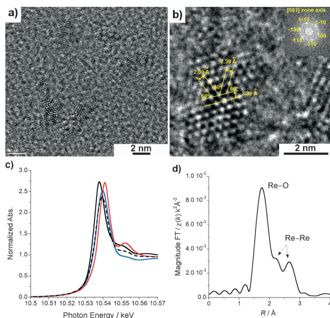
Figure 1. Identification of Re NPs. a) TEM image of Re NPs diluted in acetone and evaporated over Cu grids without interference of other supports. b) HRTEM image of hexagonal Re NPs, revealing the {1–100} crystallographic planes with a d spacing of 2.39 Å. The inset in (b) shows the FFT pattern of a single Re nanoparticle. c) Re L_3 XANES (10.50 to 10.57 keV) for \text{Re}^0 (black —), \text{ReO}_2 (blue —), and \text{NH}_4\text{ReO}_4 (red —) references, and the Re NP sample (black ---). d) EXAFS Fourier transforms of Re NPs ( \Delta k = 2.7 to 10.4 \text{ \AA}^{-1} ).
